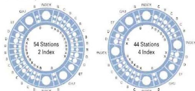
Turret Layout
